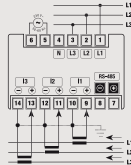
AC Three-phase
