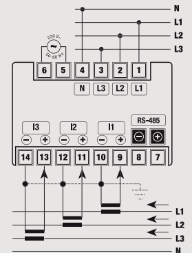
AC Three-phase + N
