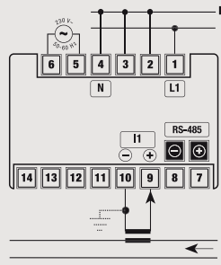
AC Single-phase
